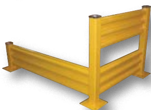
BOLT-ON STYLE model (2) YGR-LO-4, (1) YGR-TP42-S, (1) YGR-TP42-C, (1) YGR-LO-6, (1) YGR-TP18-S
