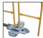
PERMANENT/ PORTABLE BASE designed to meet OSHA temporary floor edge and roof railing requirements (OSHA 1926.500) model VDKR-BASE
